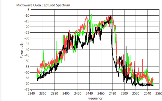
Magnetron spectral emissions in microwave oven operation – 3 traces of 30 seconds captured from same oven with the same load
