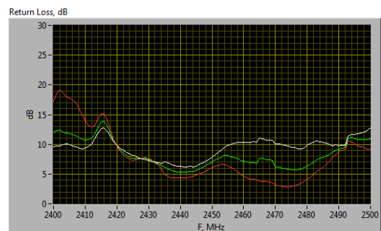
Cavity containing a distributed load of potatoes
