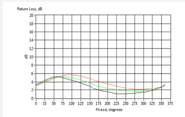
Port 1,2 and compound return loss v phase of channel 2
